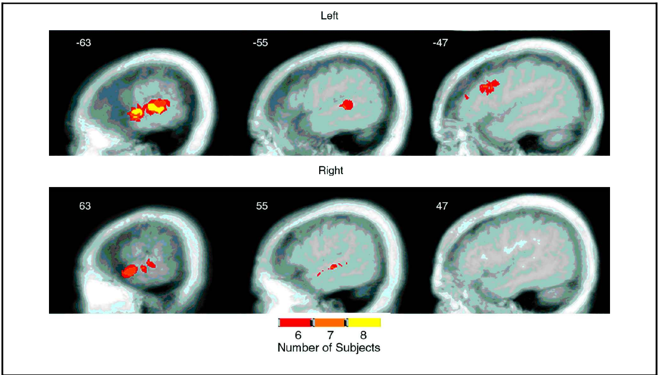
Figure 2. Speech discrimination minus tone discrimination in Experiment 2. The location of the structural images are the same as in Experiment 1. Areas showing significant activity are in the superior temporal gyrus bilaterally (see left and middle panels) and at the border of the left inferior and middle gyri (see top right panel).
